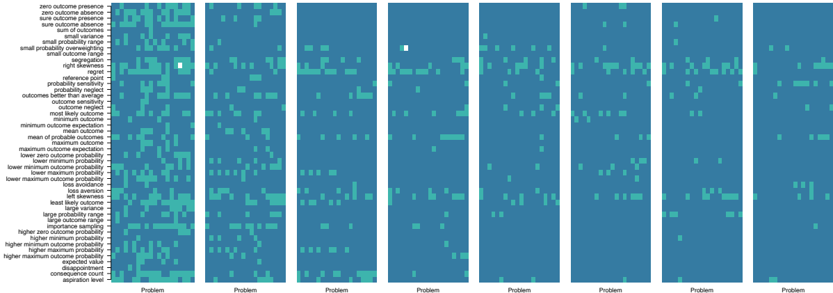
llama-31-8b M = 66.5%
