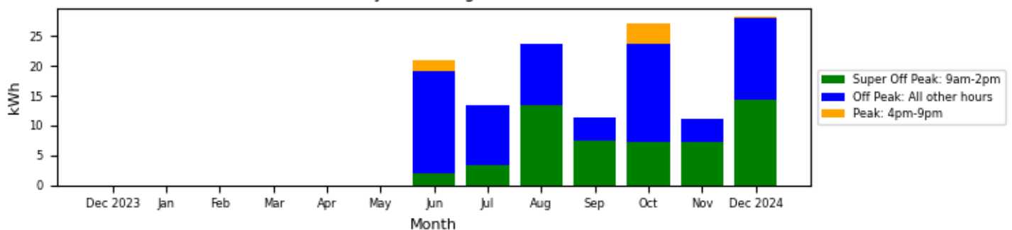
PWS-404-P06 Monthly kWh Usage Dec 2023 - Dec 2024
