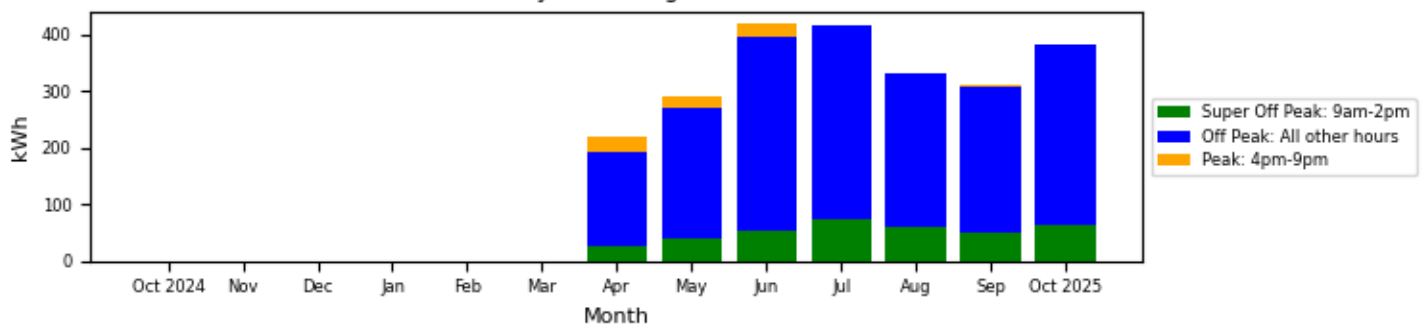
PWS-203-P07 Monthly kWh Usage Oct 2024 - Oct 2025
