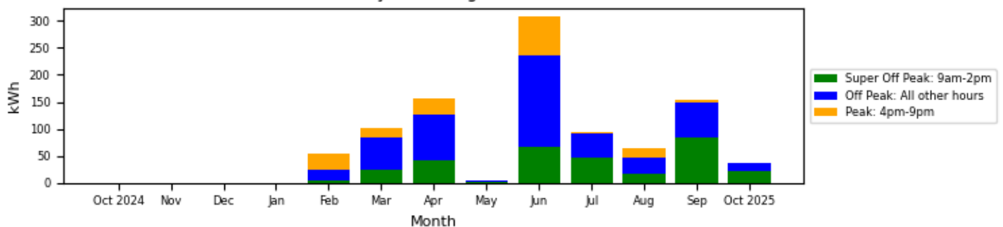
PWS-403-P20 Monthly kWh Usage Oct 2024 - Oct 2025
