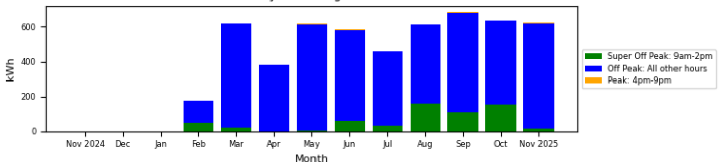
PWS-405-P14 Monthly kWh Usage Nov 2024 - Nov 2025
