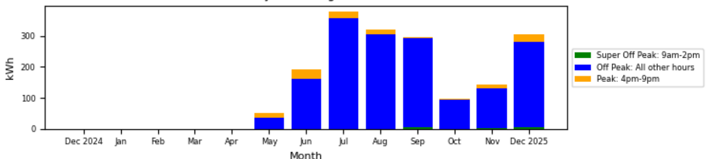
PWS-204-P26 Monthly kWh Usage Dec 2024 - Dec 2025
