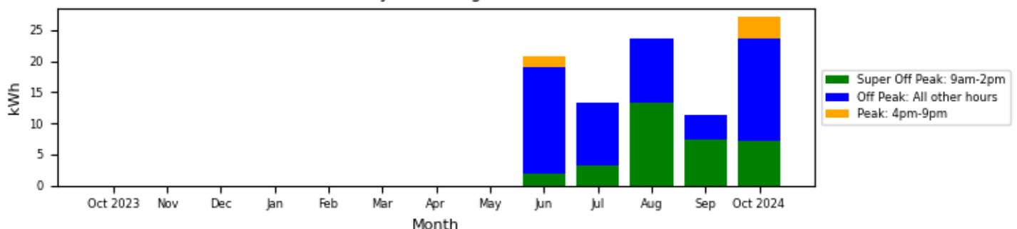
PWS-404-P06 Monthly kWh Usage Oct 2023 - Oct 2024
