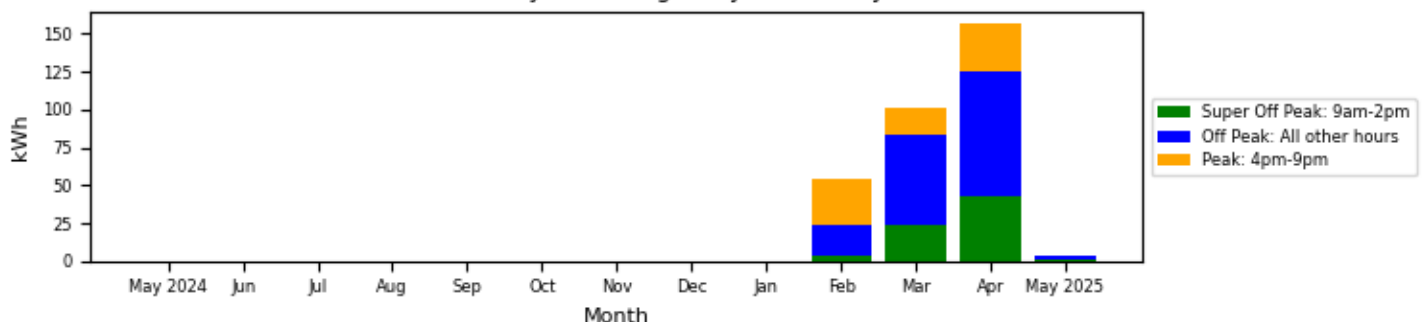
PWS-403-P20 Monthly kWh Usage May 2024 - May 2025
