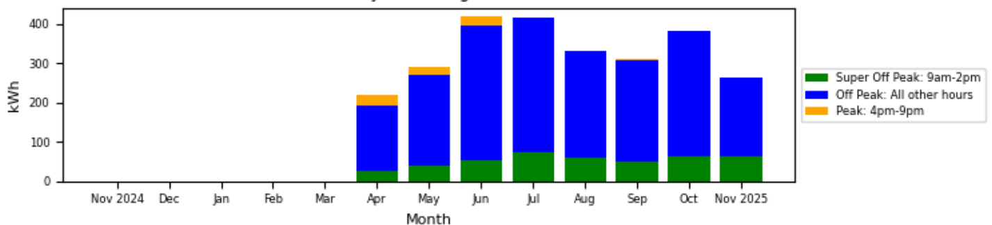
PWS-203-P07 Monthly kWh Usage Nov 2024 - Nov 2025
