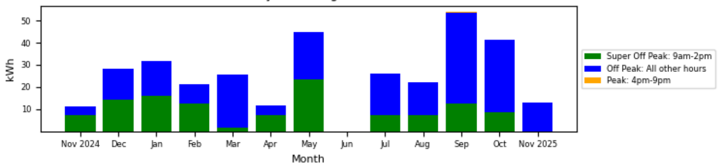
PWS-404-P06 Monthly kWh Usage Nov 2024 - Nov 2025
