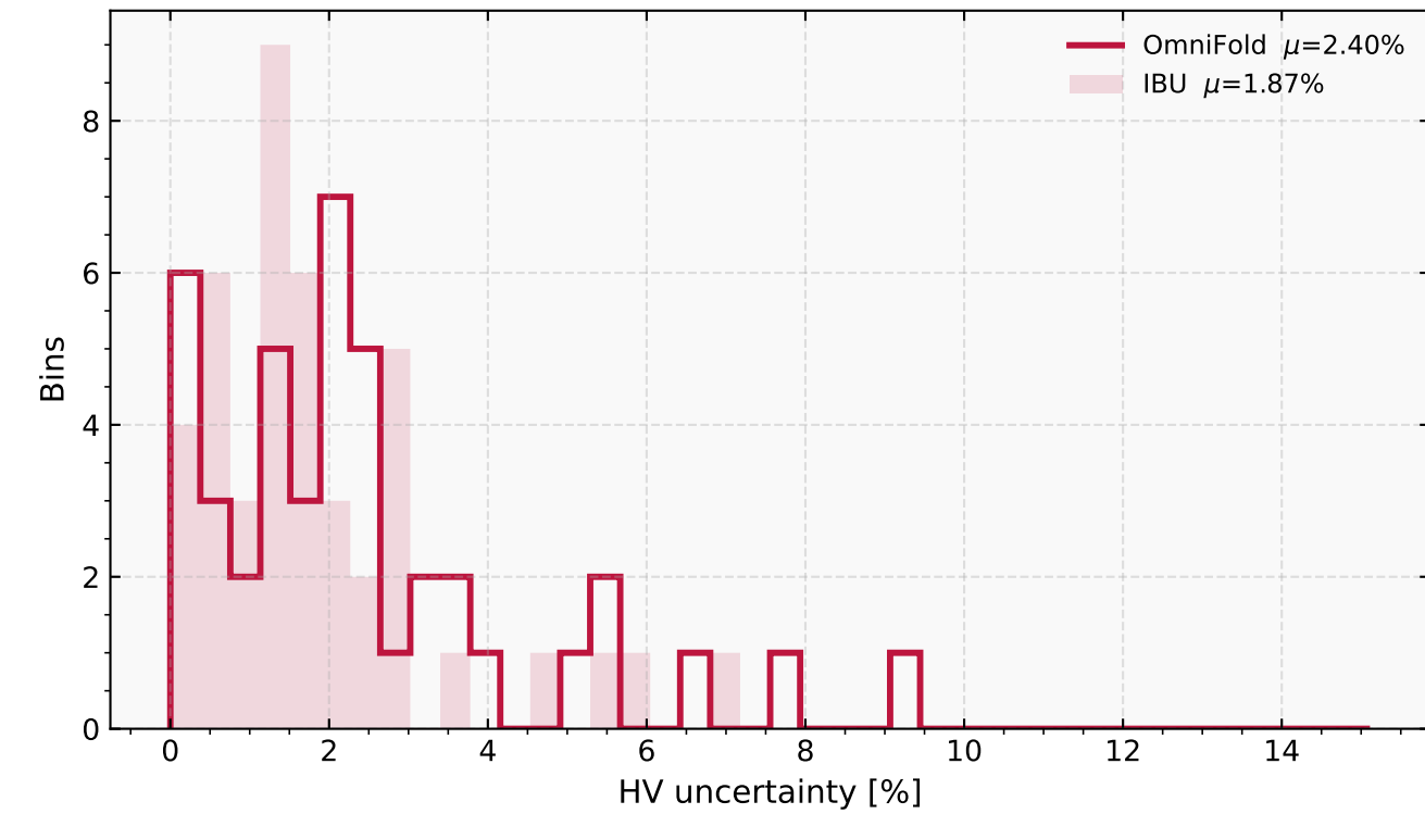
Sub-structure observables
