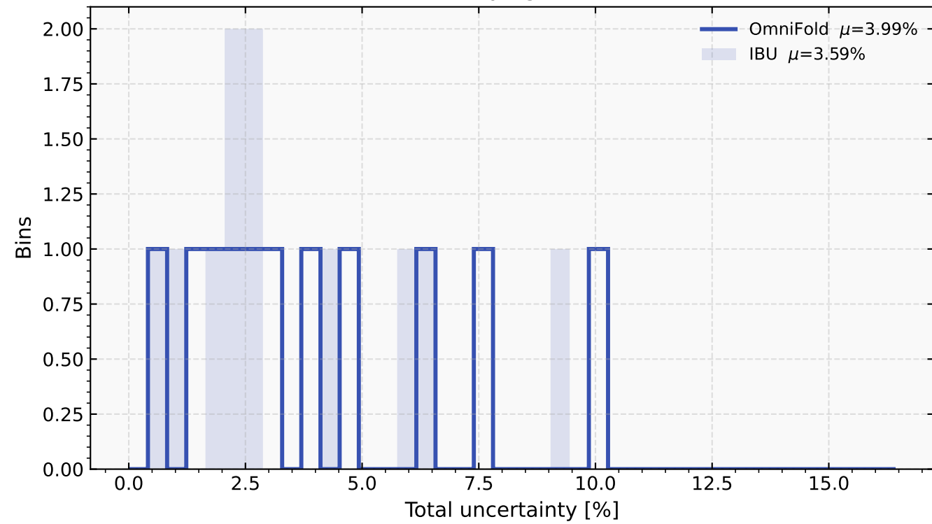
Underlying event
