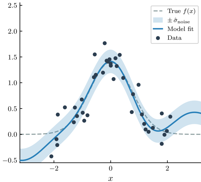
Aleatoric Uncertainty
