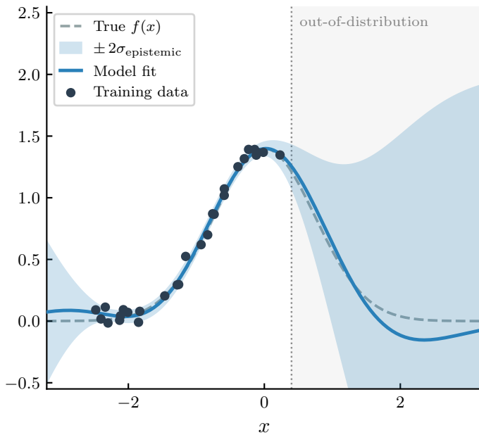
Epistemic Uncertainty
