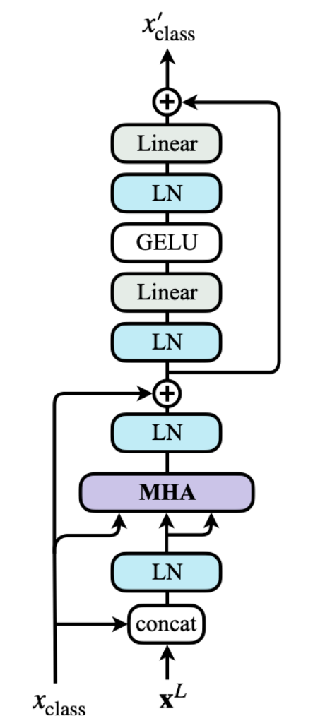
(c) Class Attention Block
