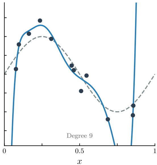
Overfitting
