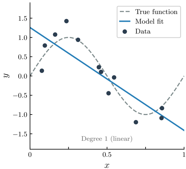
Underfitting
