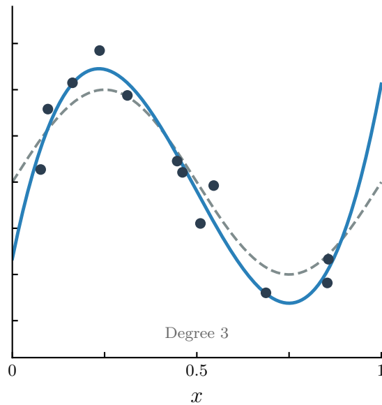
Good fit
