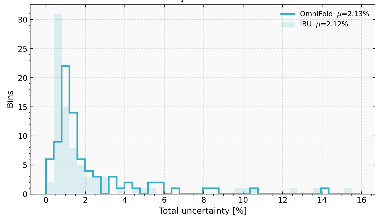
Underlying event
