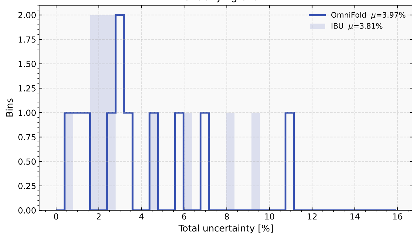
Underlying event
