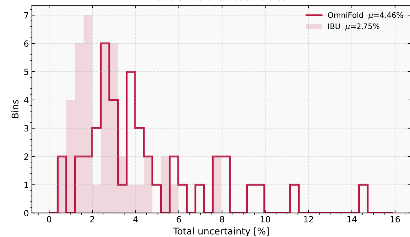
Sub-structure observables
