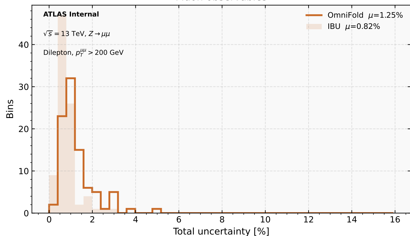
Sub-structure observables
