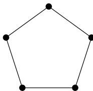
Figure 2.1 The graph C_5 made by TikZ
