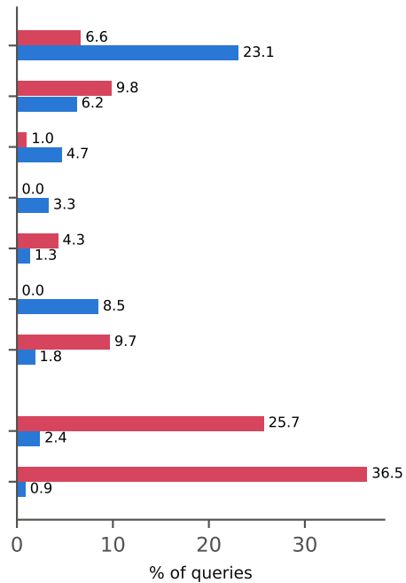
b U→W (red) and A→U (blue)
