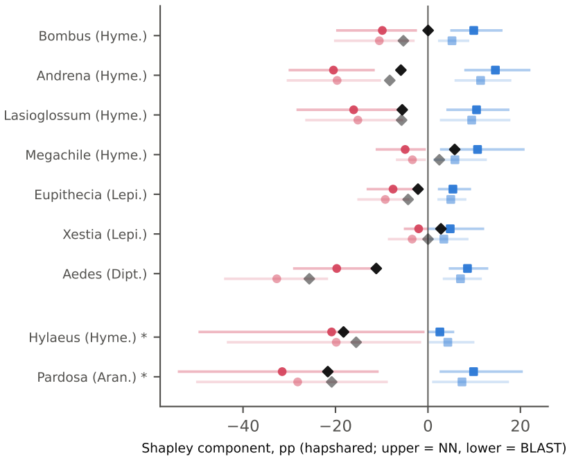
a loss (●), removal (■), net (◆)
