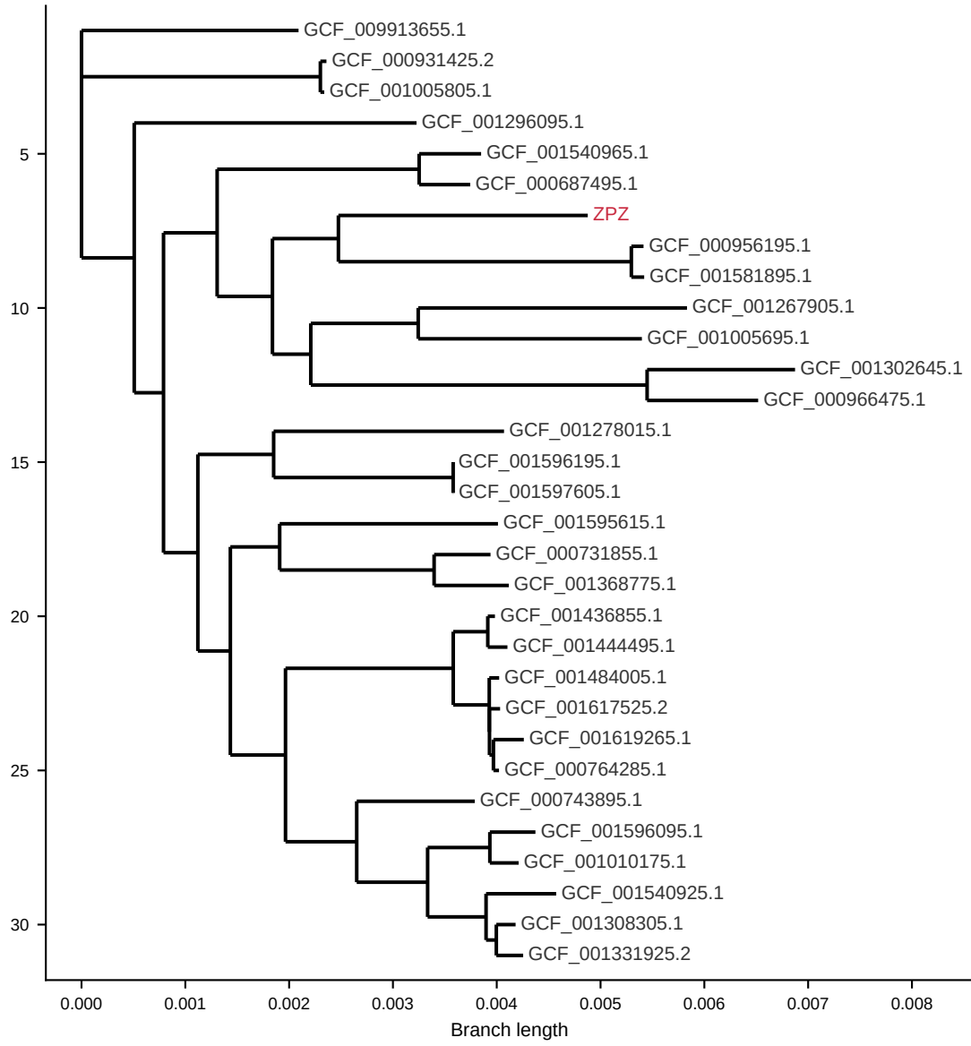
L. plantarum unrooted core-genome phylogeny
