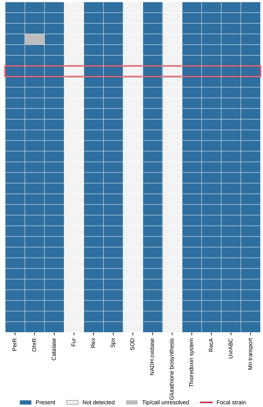
Strict 13-function genomic panel
