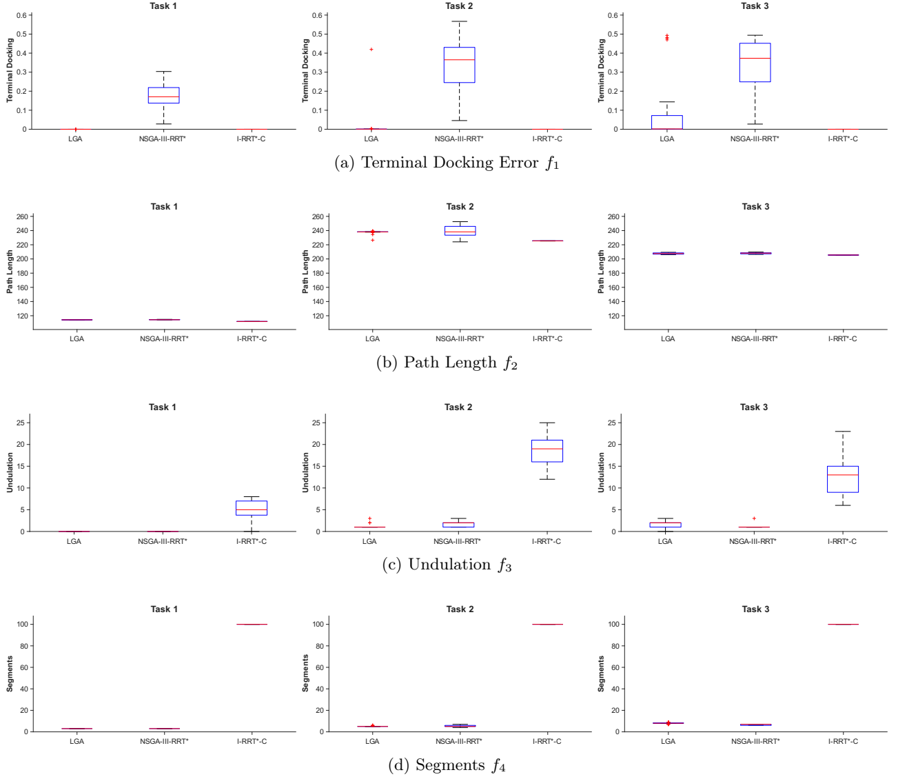
Figure S.1: Results of the four objective-function values for each algorithm across the three tasks.
