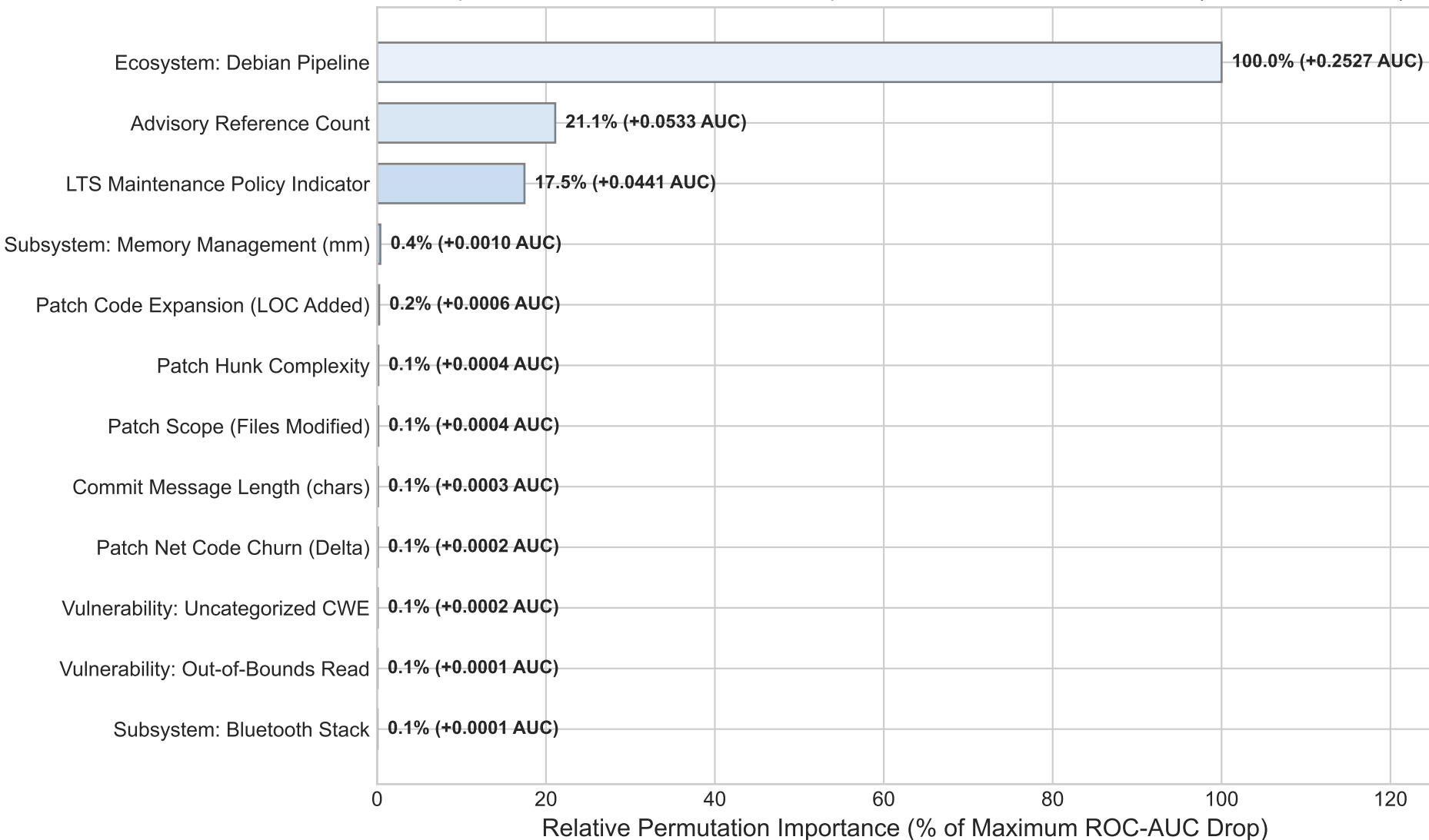
Prospective Permutation Feature Importance on Held-Out Test Set (Zero Lookahead)
