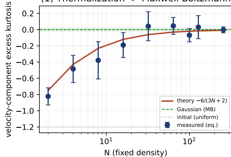
(1) Thermalization -> Maxwell-Boltzmann
