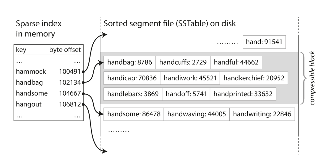
Figure 3-5. An SSTable with an in-memory index.
