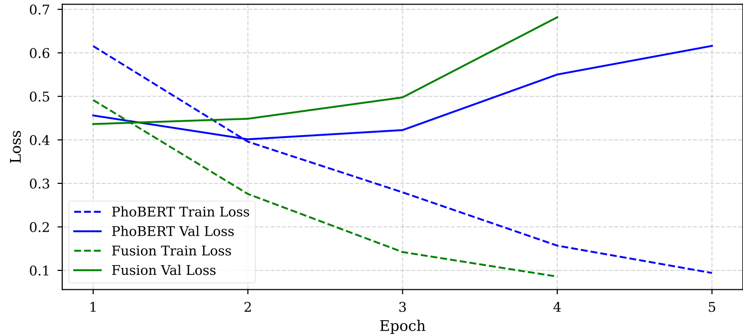
Training and Validation Loss Curves
