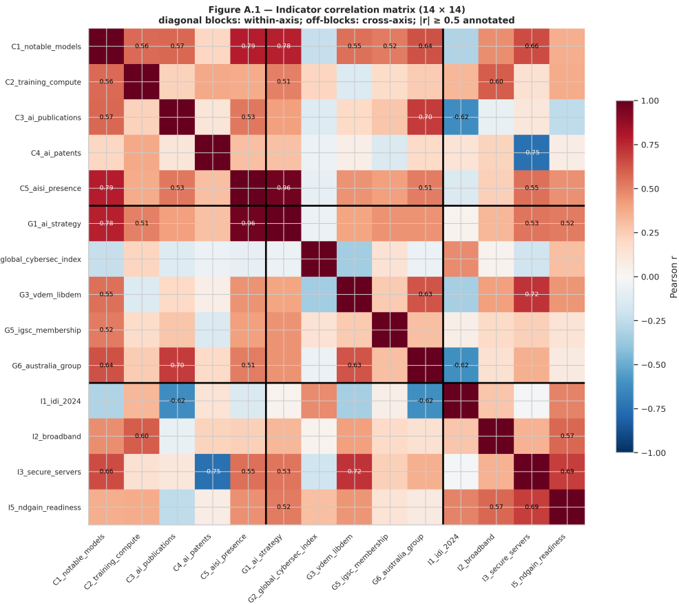
Figure 17: Full 14 × 14 indicator correlation matrix with axis-block separators; |r| \geq 0.5 annotated. Diagonal blocks are within-axis; off-blocks are cross-axis. Source: outputs/cross_axis_correlations.csv .
