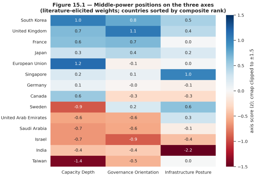
Figure 19: Per-country axis scores under the literature scheme ( z -scale, clipped to \pm 1.5 ), ordered by composite rank. Taiwan's infrastructure cell is column-mean-imputed. Source: outputs/index_baseline.csv .
