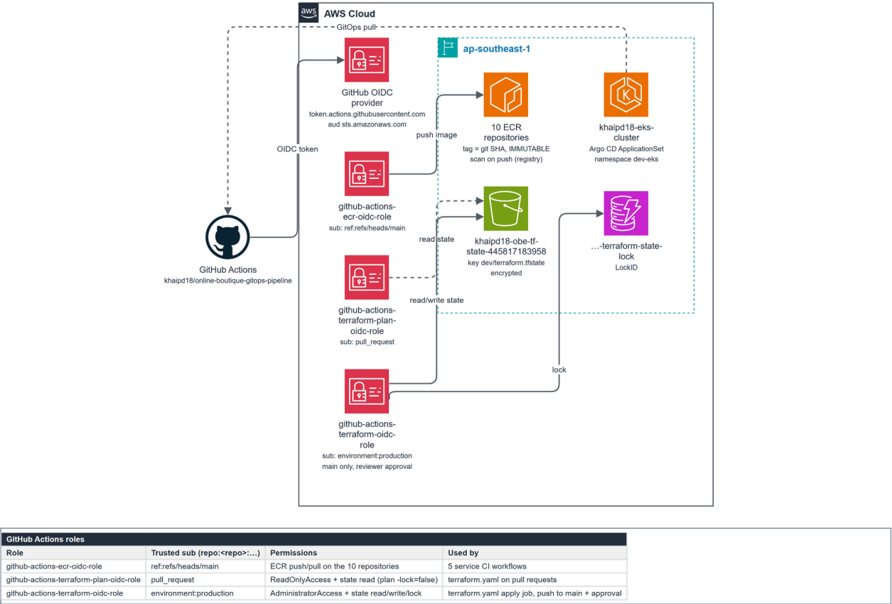
Figure 3: LLD: CI/CD and IAM OIDC
