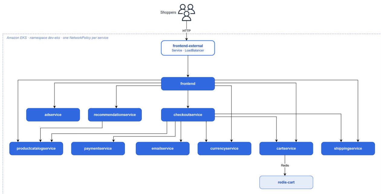
Figure 4: Calls allowed between services
