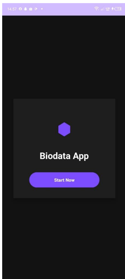
Gambar 1. Halaman Home
