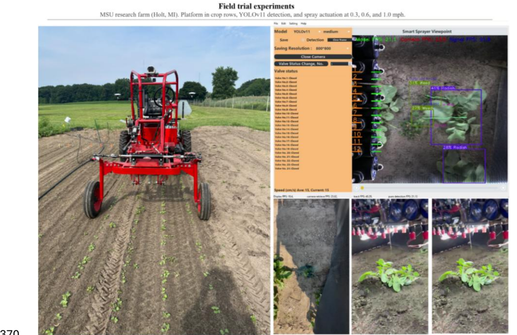
370 371 Fig. 6. Field trial experiments conducted in August 2025. Top-left: The semi-autonomous spraying platform 372 traversing radish crop rows at the MSU research farm. Top-right: Real-time software interface showing YOLOv11 373 detection output discriminating between weeds (green boxes) and radish crop (blue boxes) during field operation. 374 Bottom row (left to right): Close-up of inter-row weed populations targeted during trials; blue dye deposition on soil 375 and plant surfaces following a sprayer pass; radish canopy at the 5–7 true-leaf stage present during spray trials.
