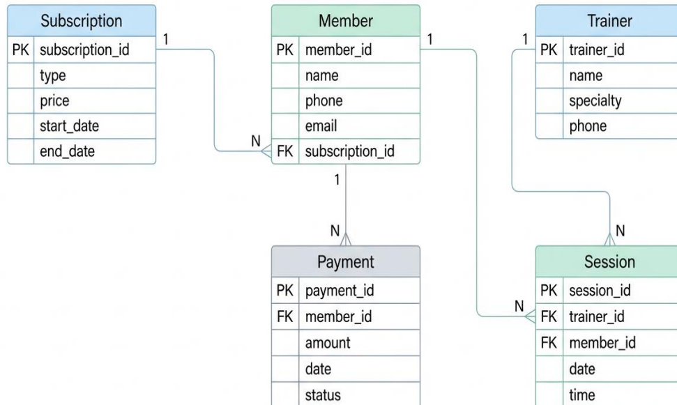
Database Schema Diagram - Gym Management System
