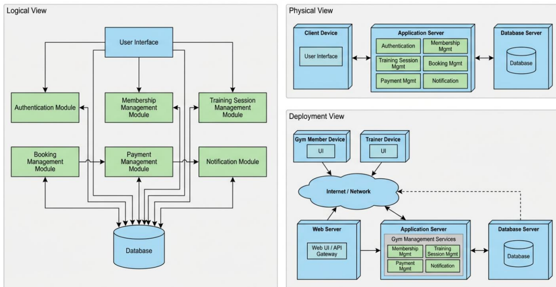
UML Architecture View Diagram "Gym Management System"
