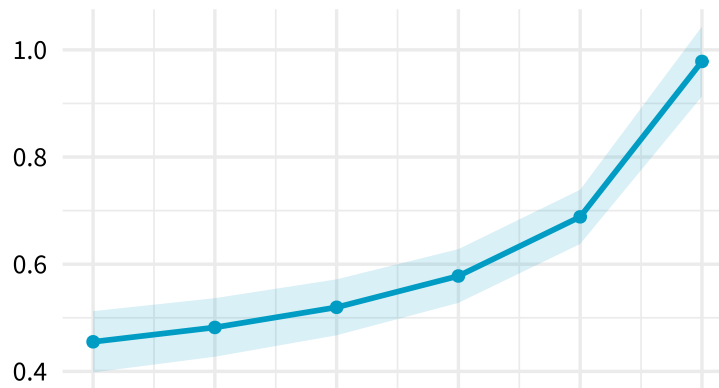
RRMSE( \beta )
