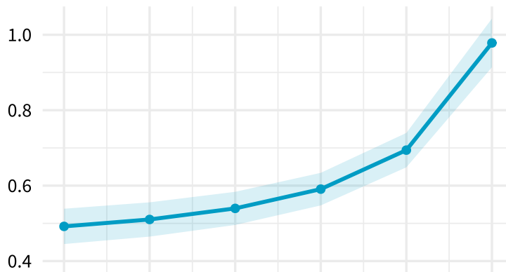
RRMSE( \Gamma )
