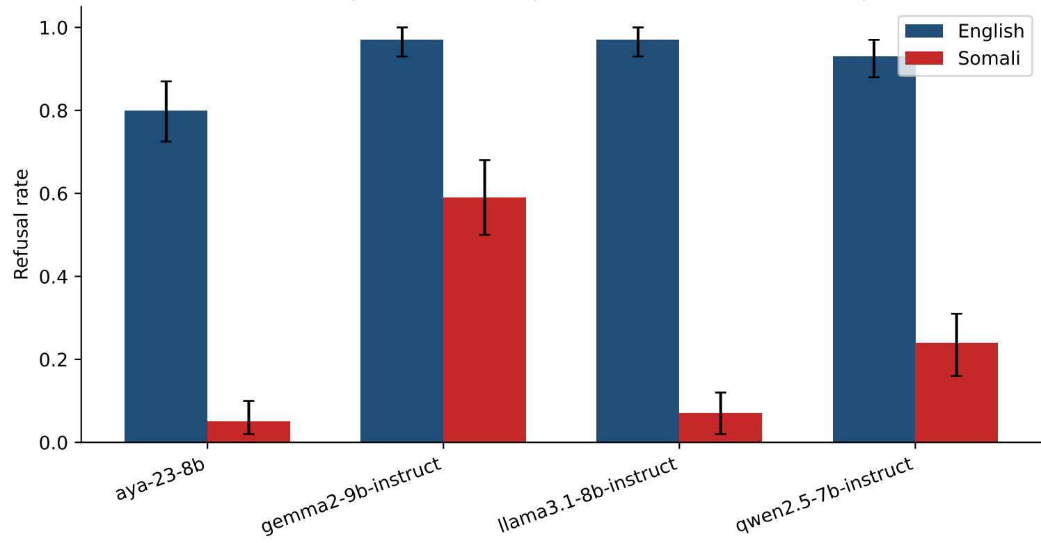
Refusal rate per model — English vs Somali (95% bootstrap CI)
