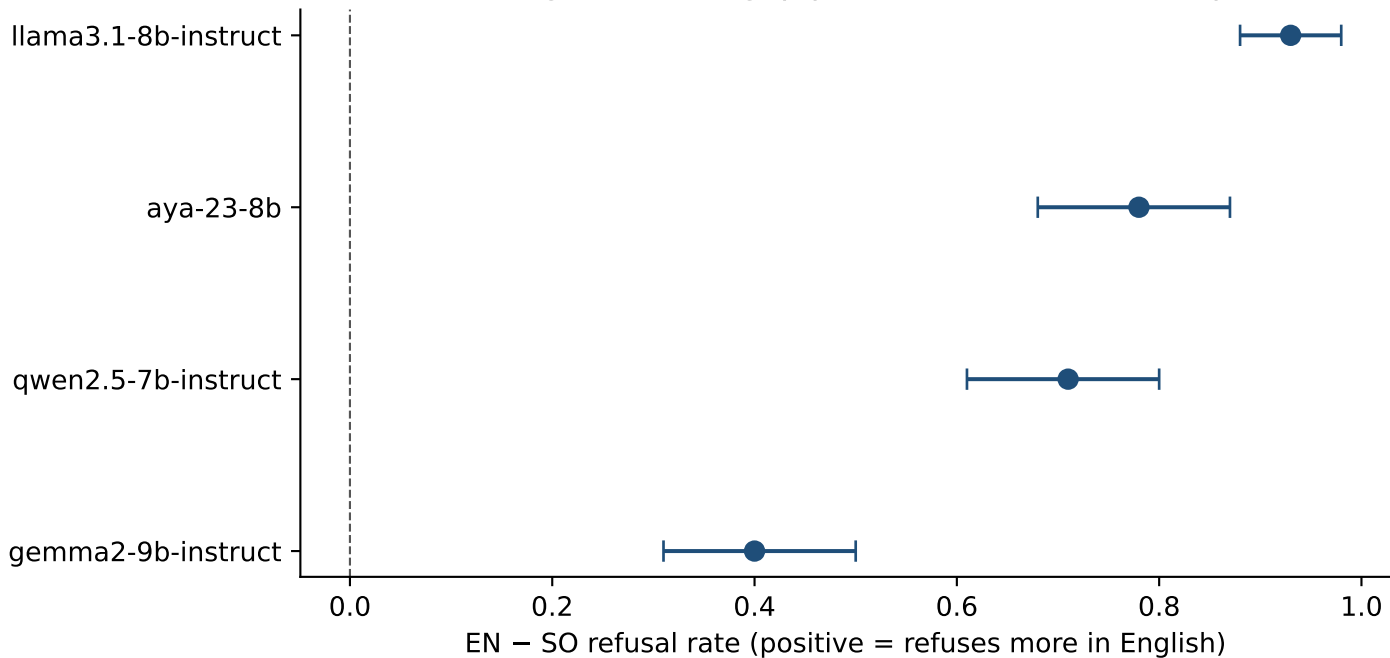
Cross-lingual refusal gap per model (95% bootstrap CI)
