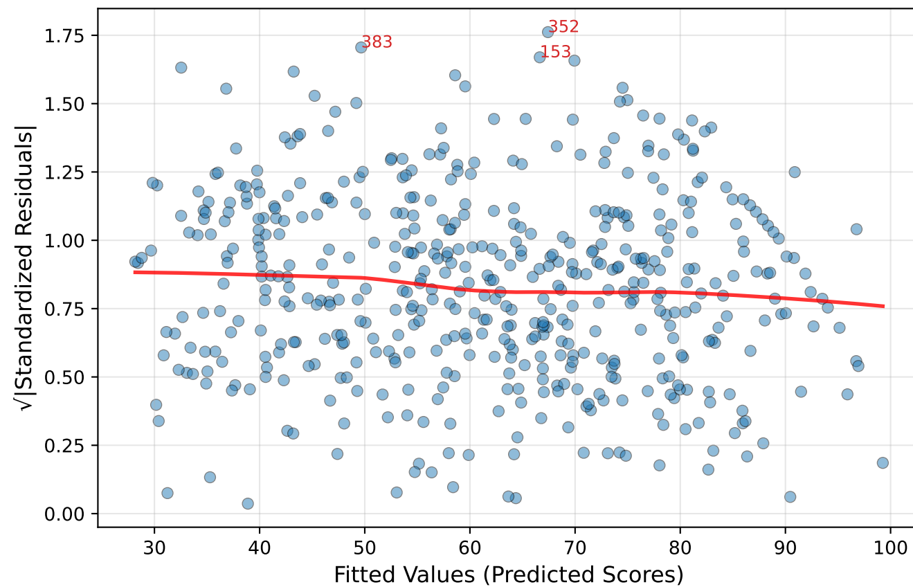
Scale-Location
