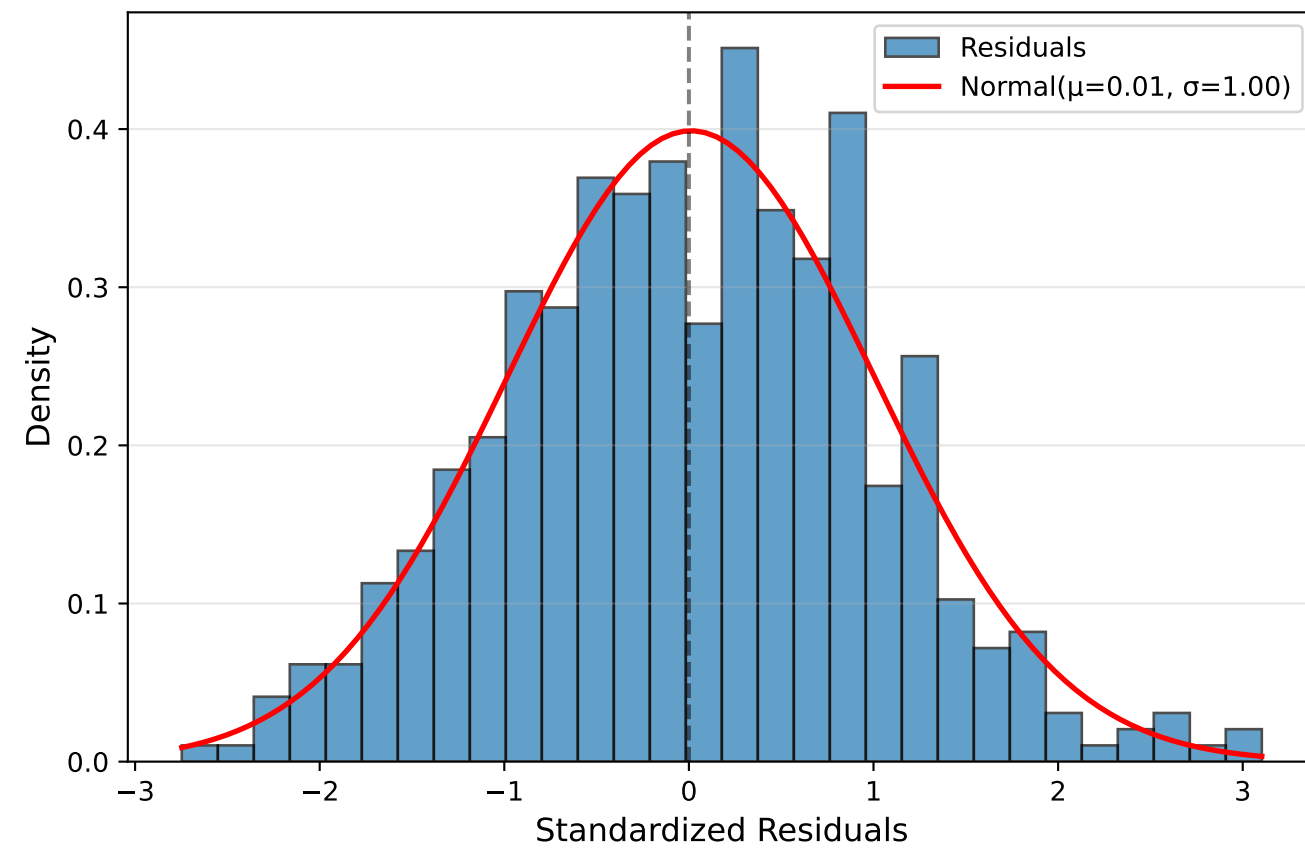
Residual Distribution
