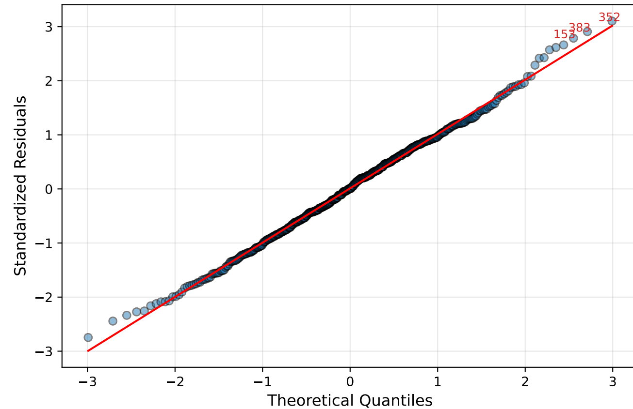
Residual Distribution
