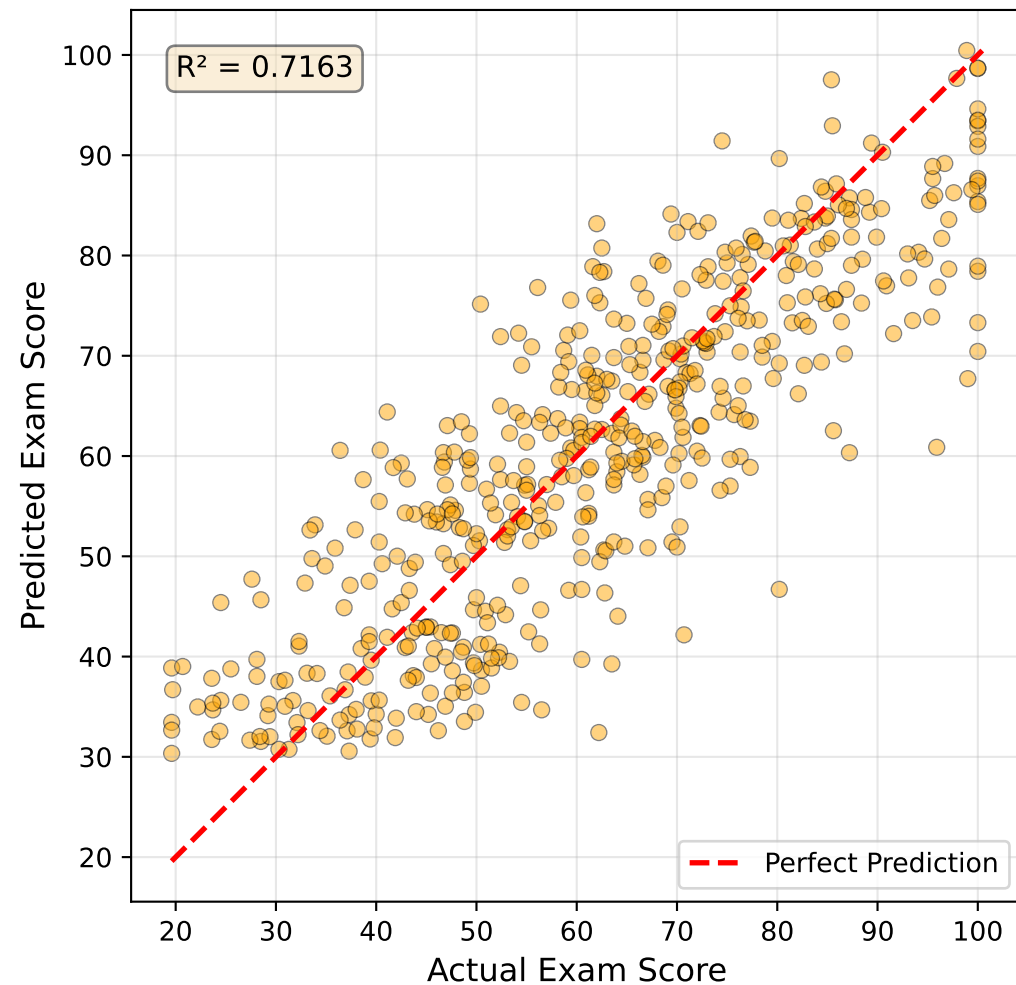
Test Set (n=500)
