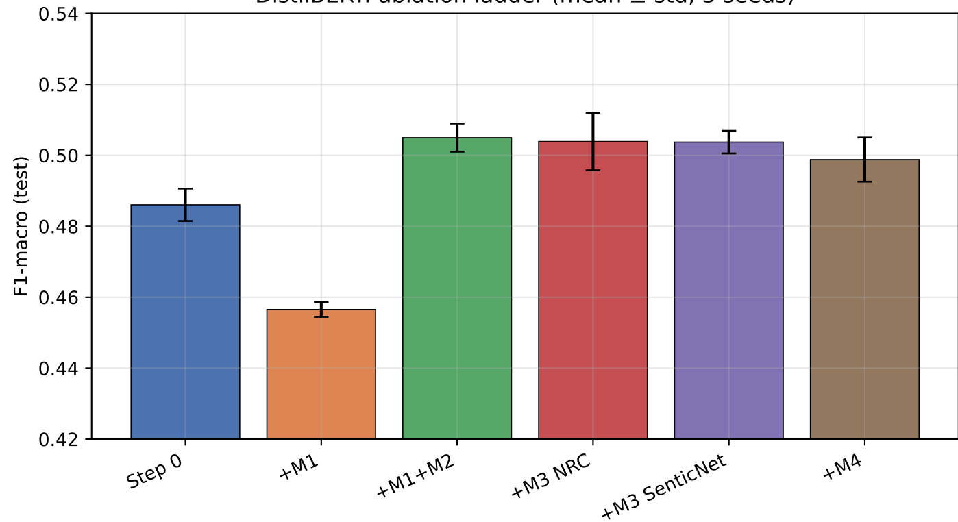
DistilBERT: ablation ladder (mean \pm std, 3 seeds)
