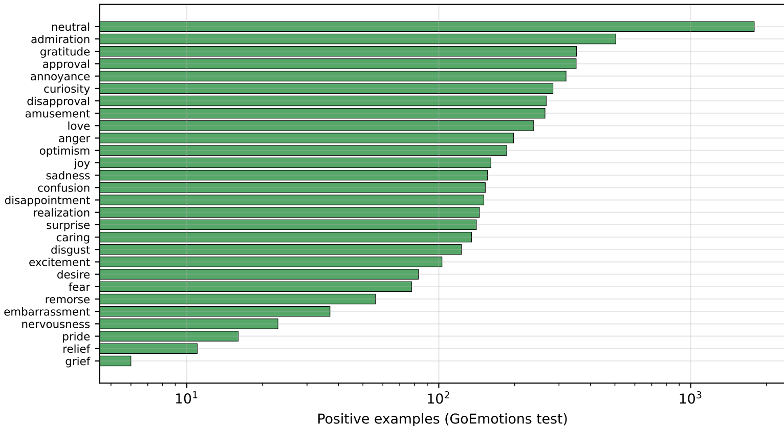
Long-tail label support (test split)
