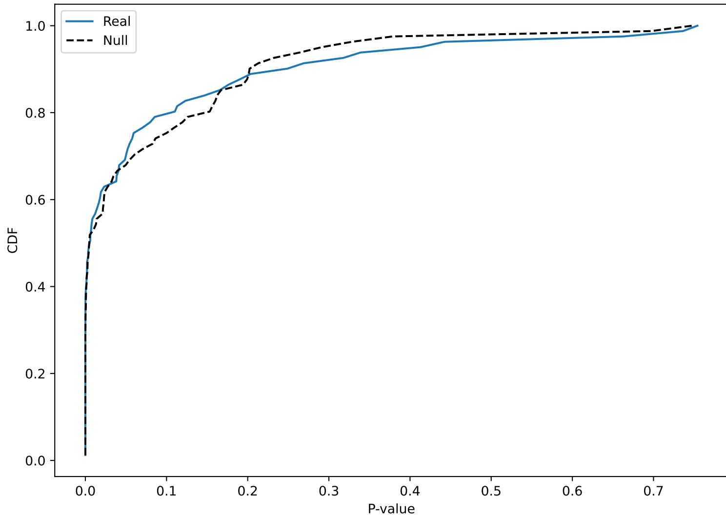
CDF of P-values — AVG-based
