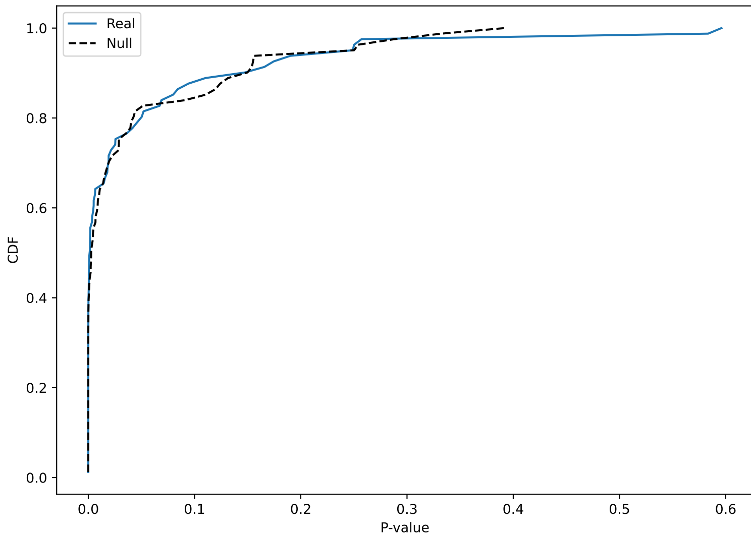
CDF of P-values — P-value-based
