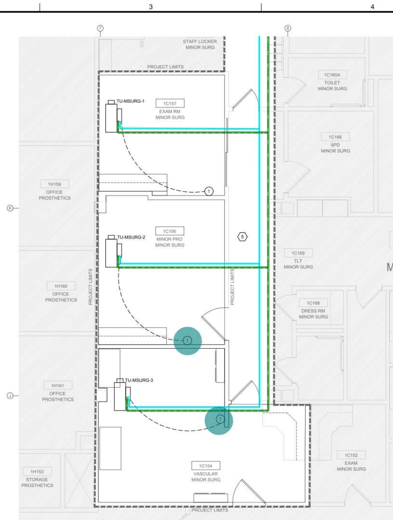
C2 FIRST FLOOR PIPING PLAN SCALE: 1/4" = 1'-0"
