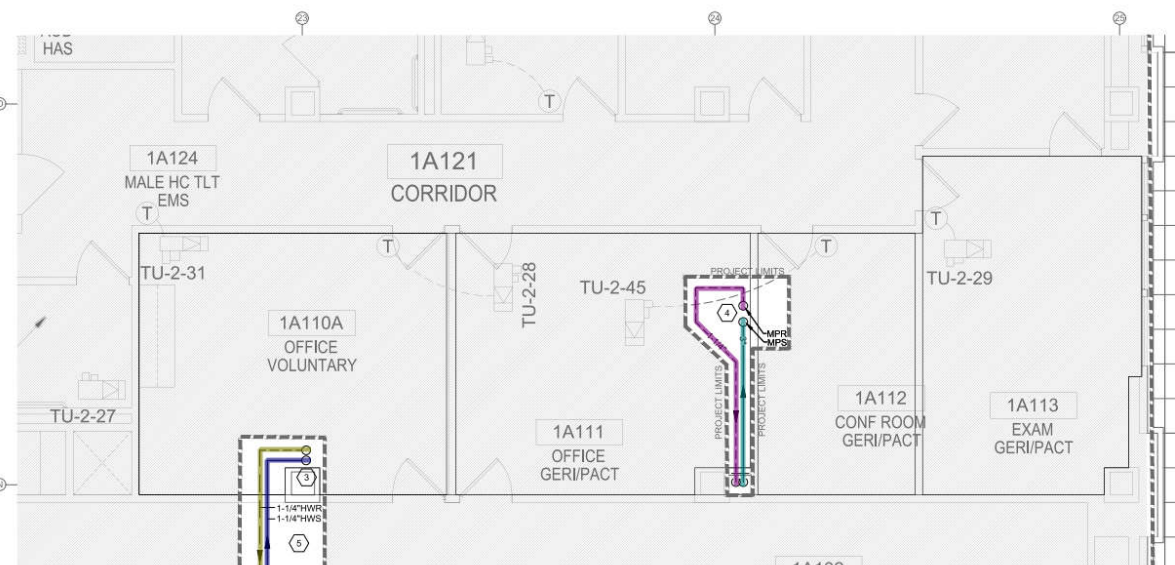
D2 FIRST FLOOR PIPING PLAN SCALE: 1/4" = 1'-0"
