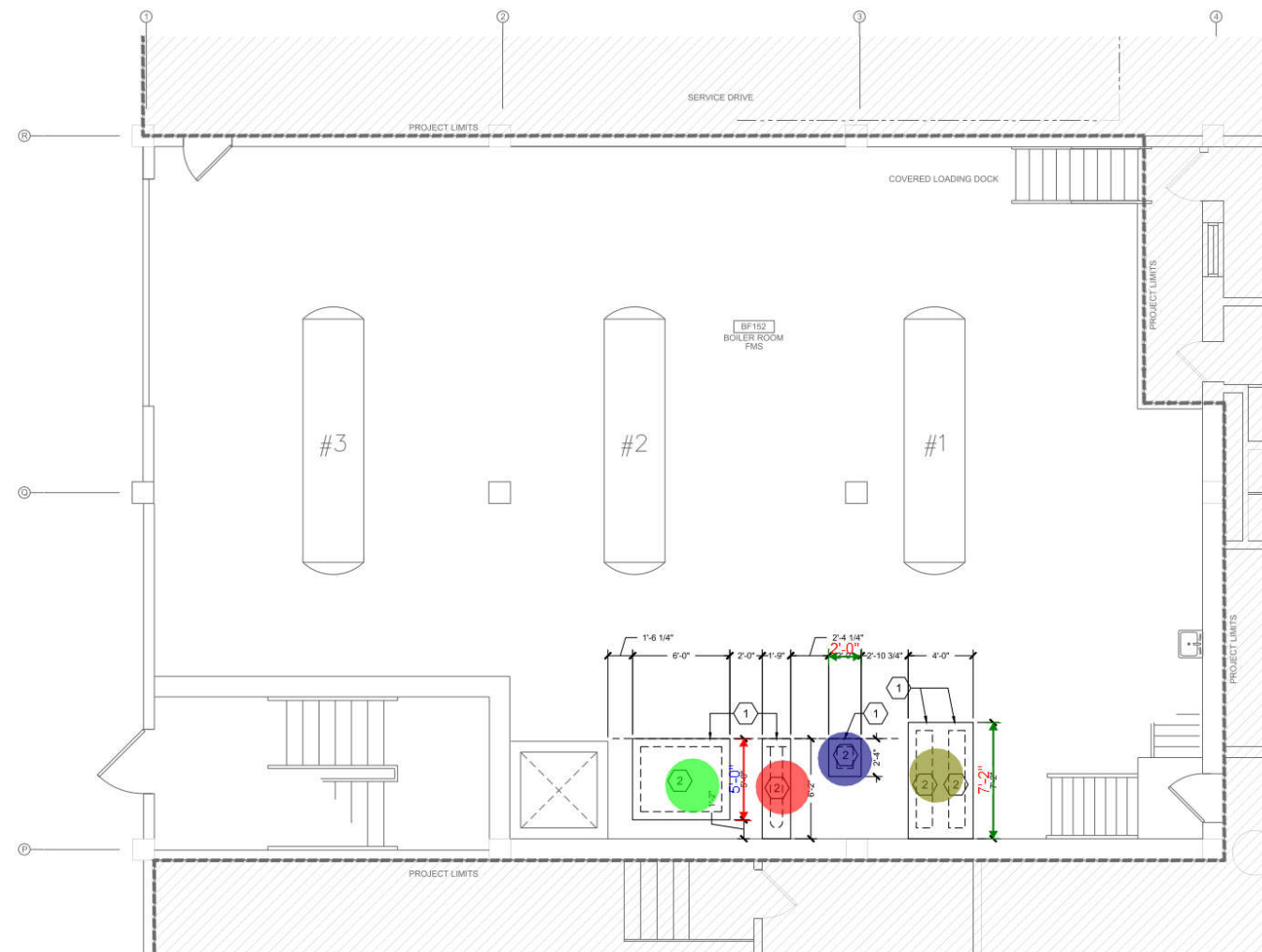
C1 BASEMENT FLOOR PLAN SCALE: 1/4" = 1'-0" 0' 2' 4' 4' 0 1/4"
