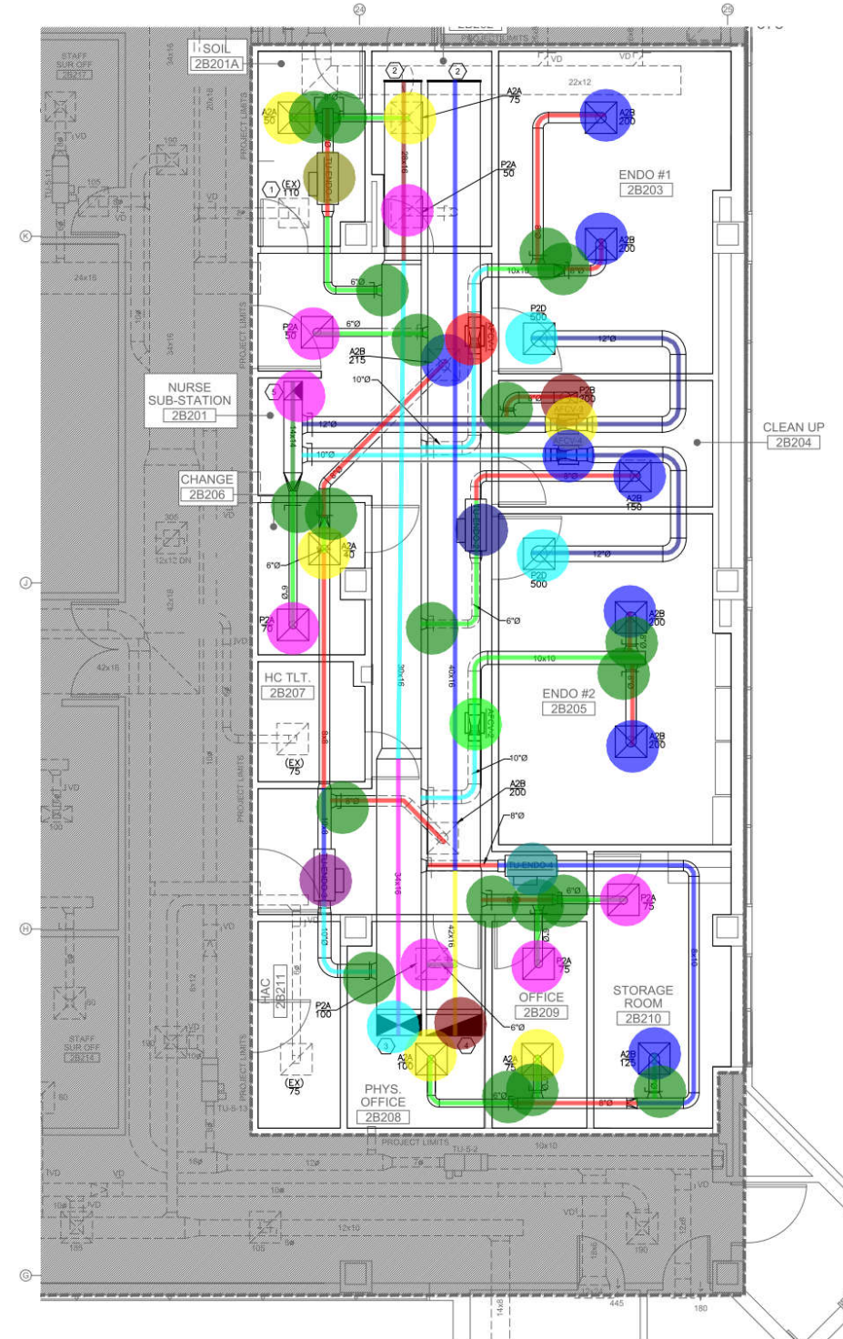
D3 SECOND FLOOR DUCT PLAN SCALE: 1/4" = 1'-0"
