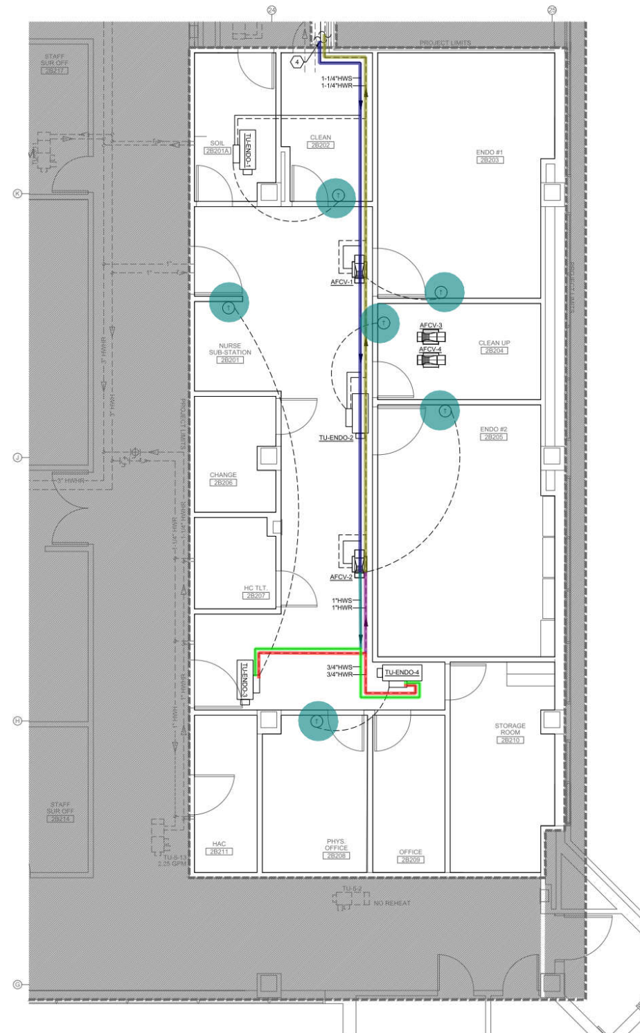
D3 SECOND FLOOR PIPING PLAN SCALE: 1/4" = 1'-0"
