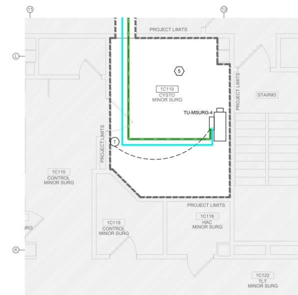
B4 FIRST FLOOR PIPING PLAN SCALE: 1/4" = 1'-0"
