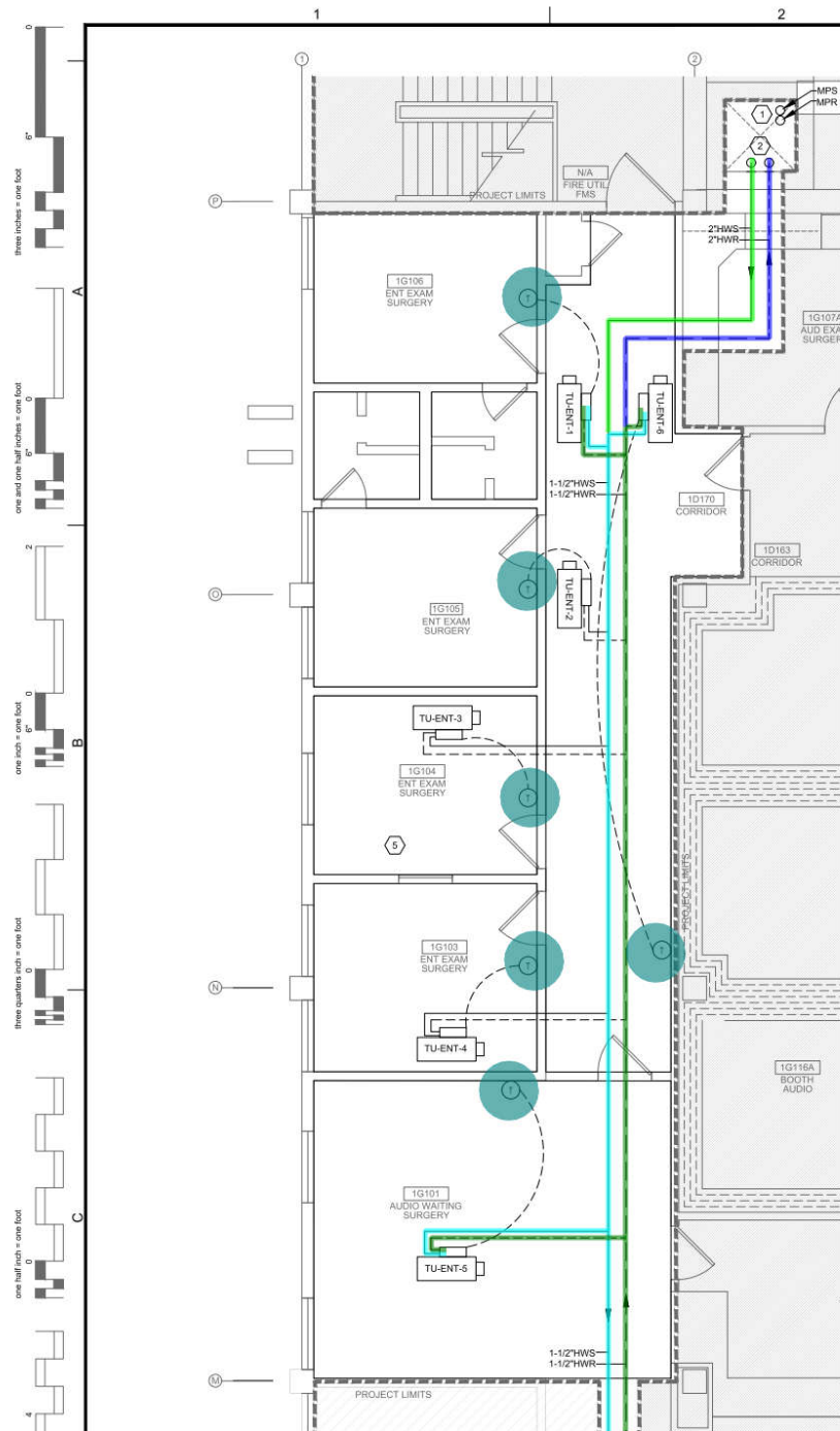
C1 FIRST FLOOR PIPING PLAN SCALE: 1/4" = 1'-0"
