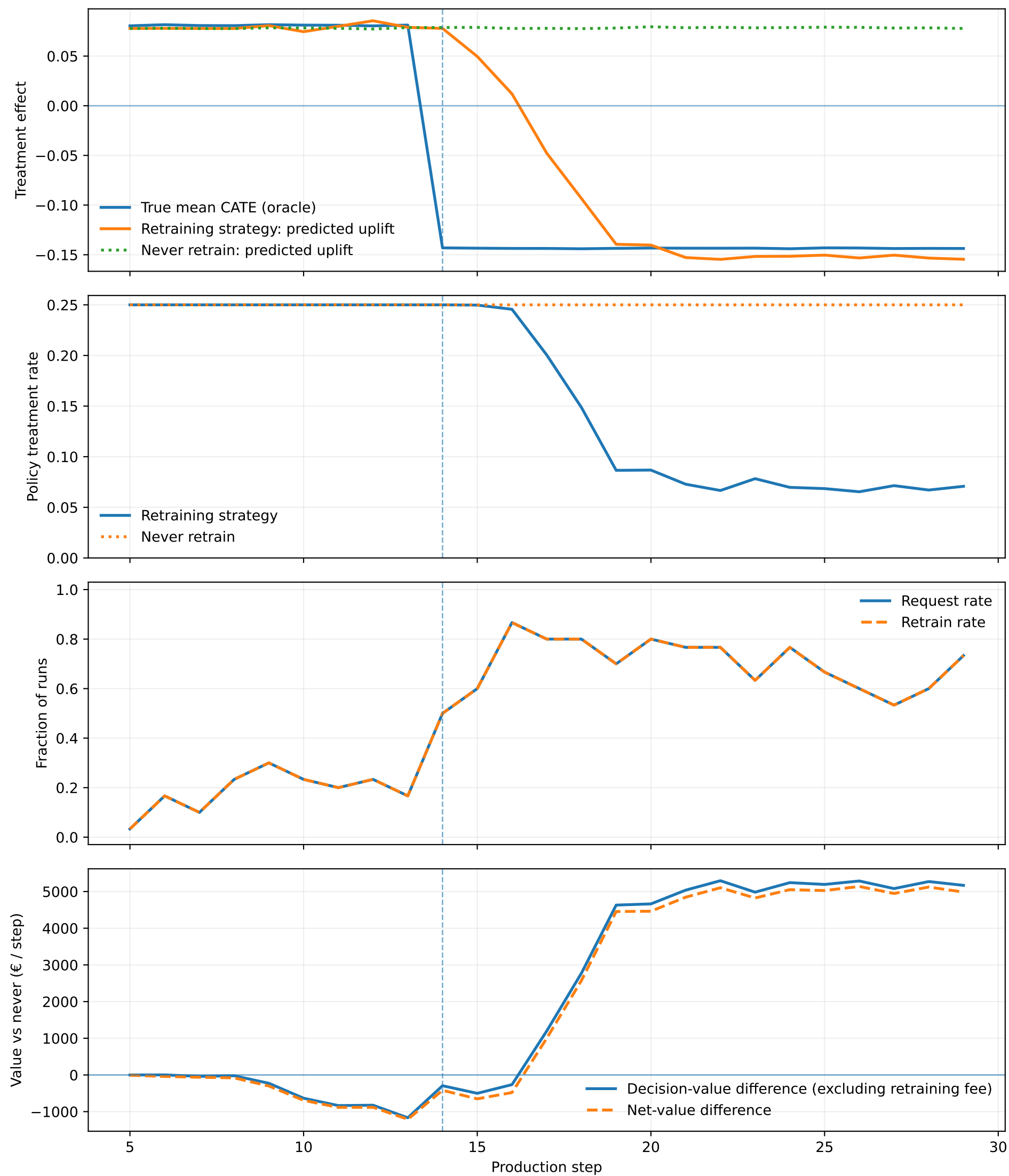
Persistent treatment-effect drift: causal adaptation creates value
