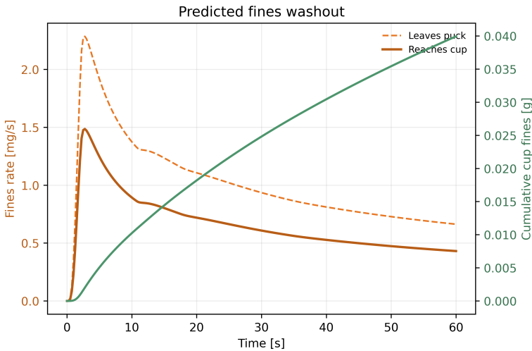
New Darcy run with exponential permeability; constant basket retention.
