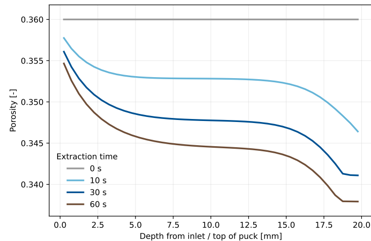
Model t = 0 : start of saturated extraction; dry/preinfusion not modeled.
