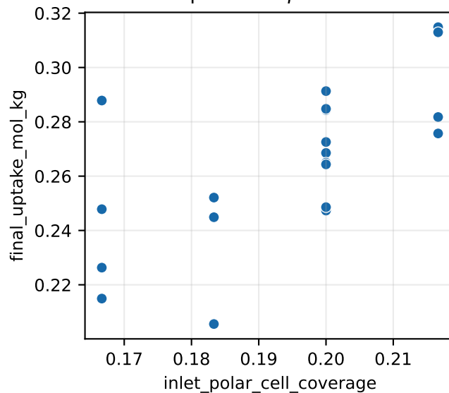
Spearman \rho=0.64
