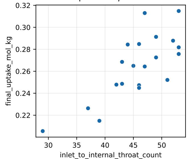
Spearman \rho=0.70
