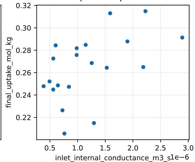
Spearman \rho=0.55
