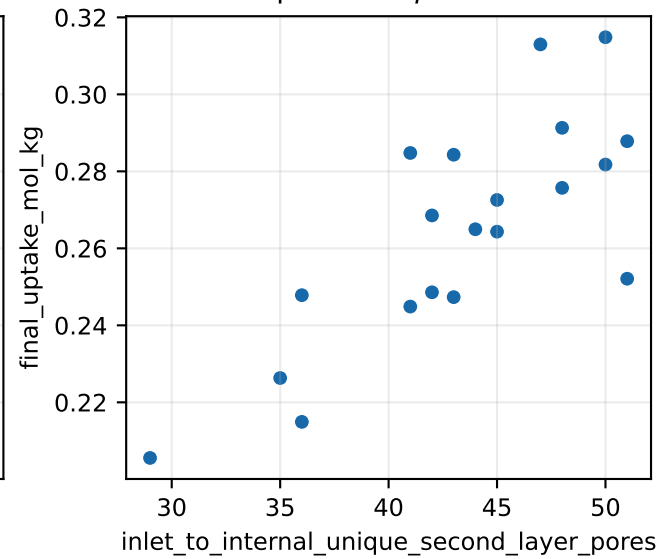
Spearman \rho=0.55
