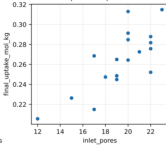
Spearman \rho=0.64
