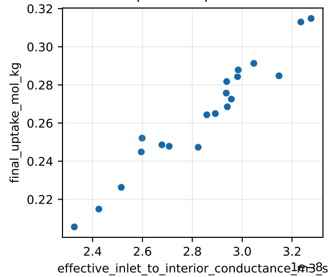
Spearman \rho=0.70
