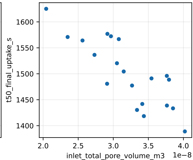
Spearman \rho=-0.54
