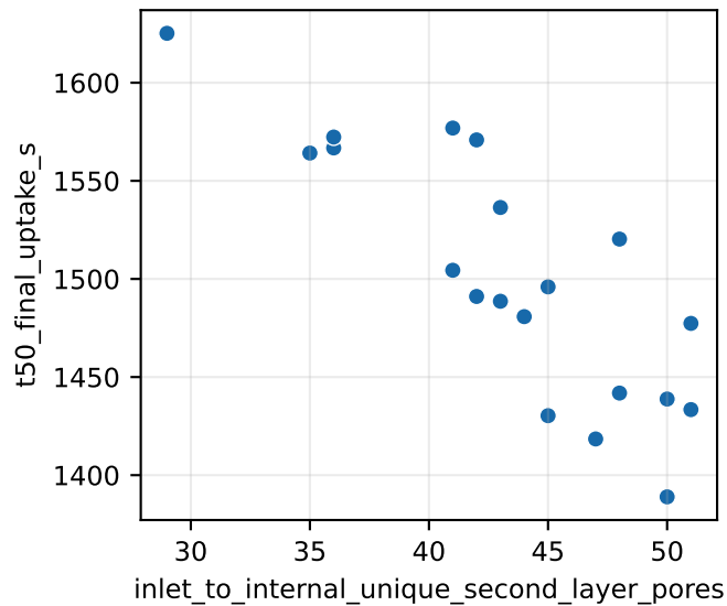
Spearman \rho=-0.77
