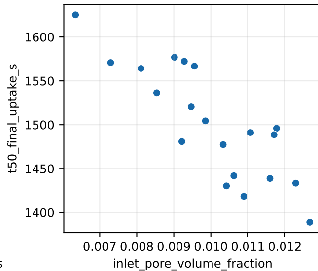
Spearman \rho=-0.74
