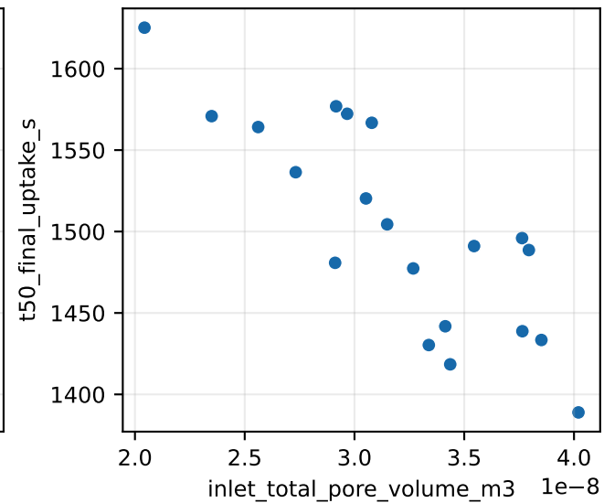
Spearman \rho=-0.54
