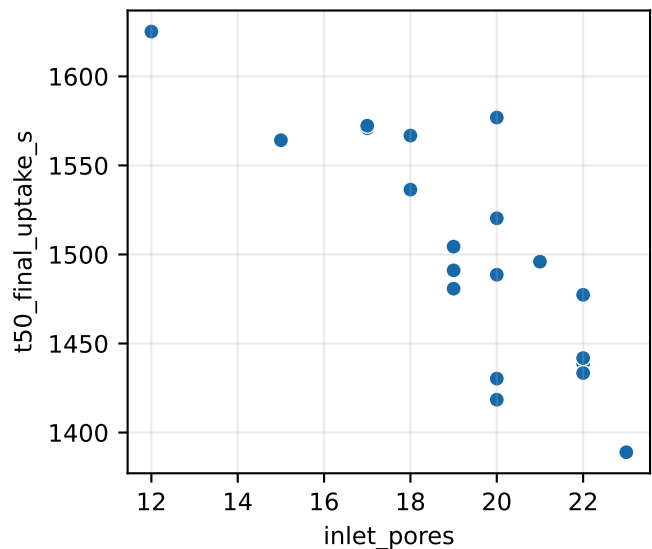
Spearman \rho=-0.77
