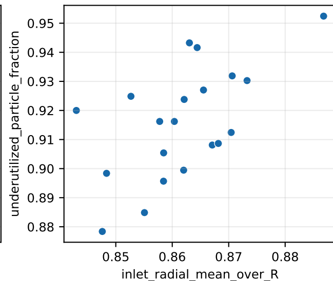
Spearman \rho=0.56
