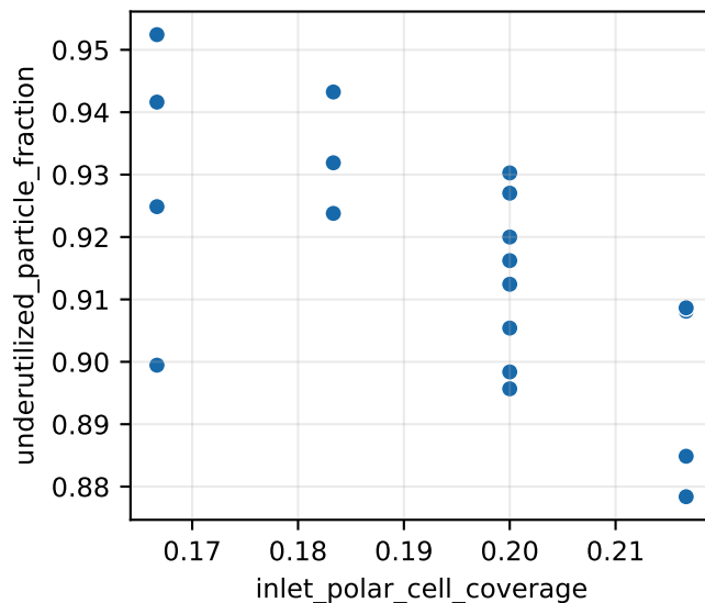
Spearman \rho=-0.64
