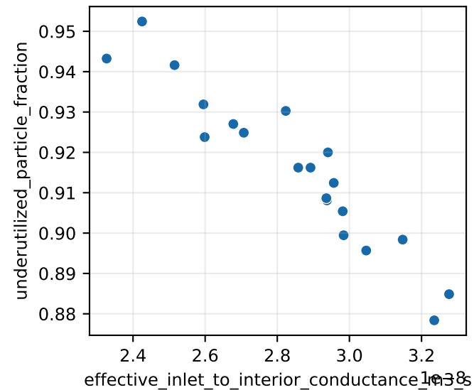
Spearman \rho=-0.68
