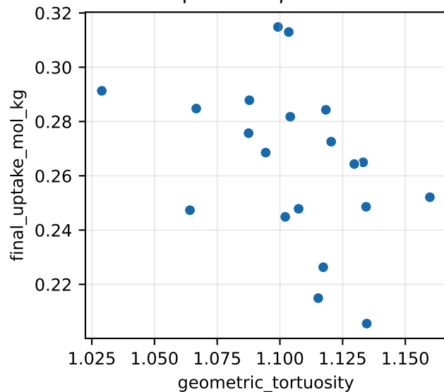
Spearman \rho=0.23
