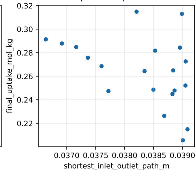
Spearman \rho=-0.21
