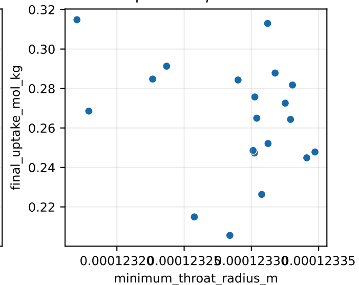
Spearman \rho=-0.21
