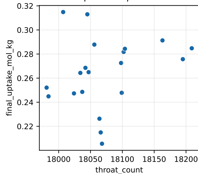
Spearman \rho=0.25
