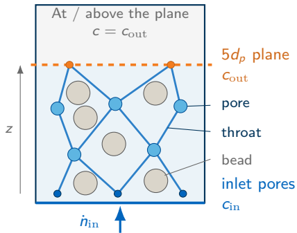
Schematic pore network
