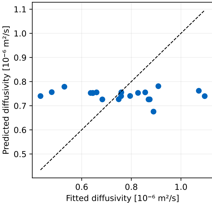
Particle GNN
