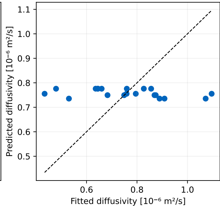
Mean diffusivity
