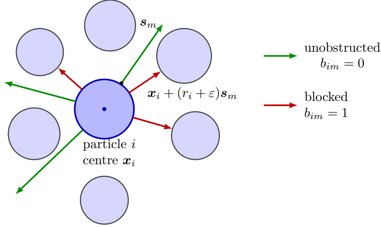
Figure 3: Schematic of the ray-tracing calculation for one particle i . Rays start just outside its surface and follow sampled outward directions \mathbf{s}_m . A ray is blocked when it intersects another particle; otherwise, it contributes to the exposed fraction. For clarity, only a two-dimensional section and a small subset of rays are shown; the actual calculation distributes M = 512 directions over the complete sphere.
