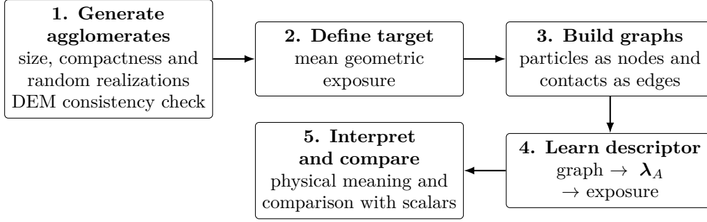
Figure 1: Five-step workflow for generating synthetic agglomerates, representing them as graphs, learning a compact structural descriptor and evaluating its physical meaning and predictive value. DEM is an auxiliary consistency check within generation, not a separate characterization step. The learning and comparison stages remain pending for the new dataset.
