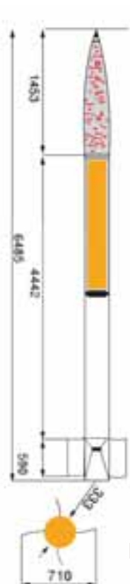
FADJR 5 ROCKET
